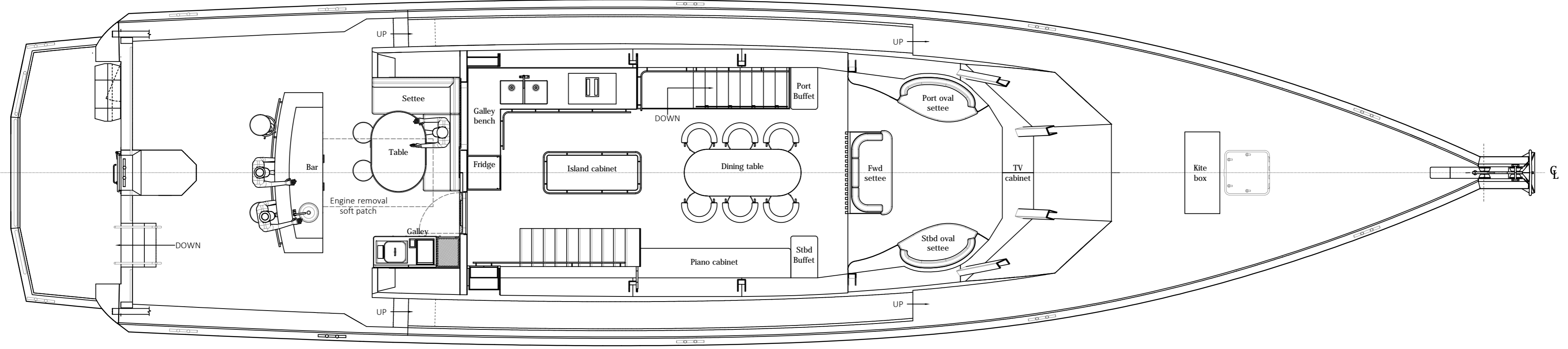
MAIN DECK
