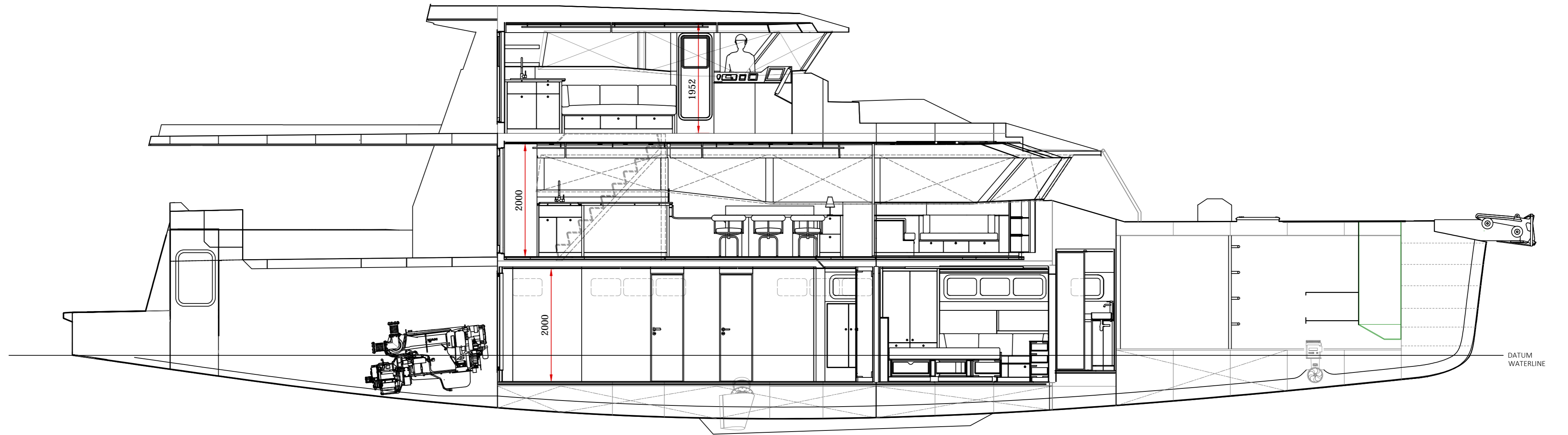
INBOARD PROFILE
